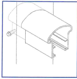
Routed Post
