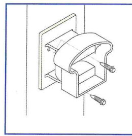
Horizontal Bracket
